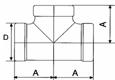
. Tee F/F/F Ref. 2003
