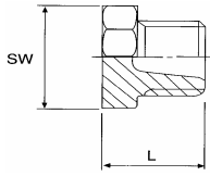
. Hexagon plug Ref. 2022 or 2023 (plain)
