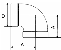
. Elbow 90° F/F Ref. 2001
