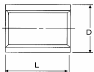
. Socket bright Ref. 2015
